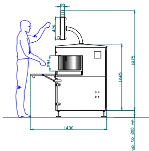
side view - vista laterale
