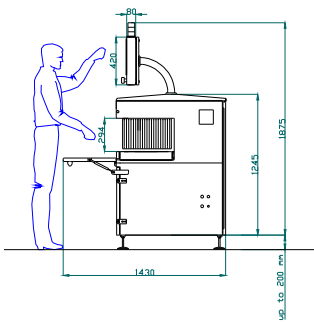
side view - vista laterale
