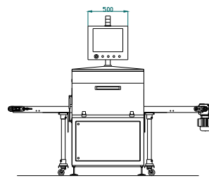
front view - vista frontale
